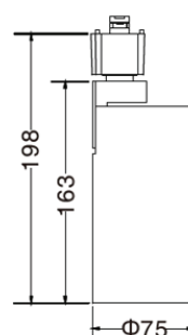
3-pin track adaptor
