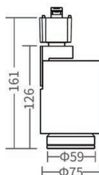
3-pin track adaptor
