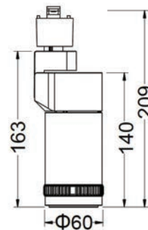
3-pin track adaptor
