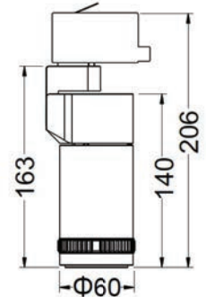
4-pin track adaptor
