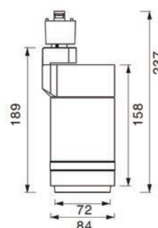
3-pin track adaptor
