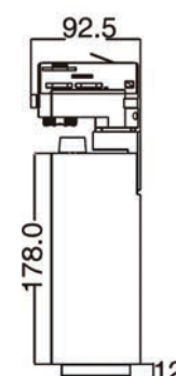
4-pin track adaptor
