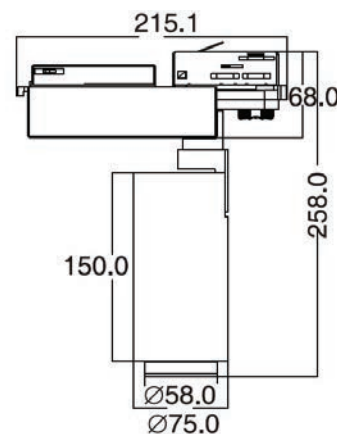
4-pin track adaptor
