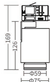
4-pin track adaptor
