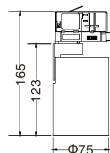
4-pin track adaptor
