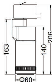
4-pin track adaptor
