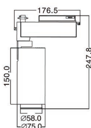
3-pin track adaptor
